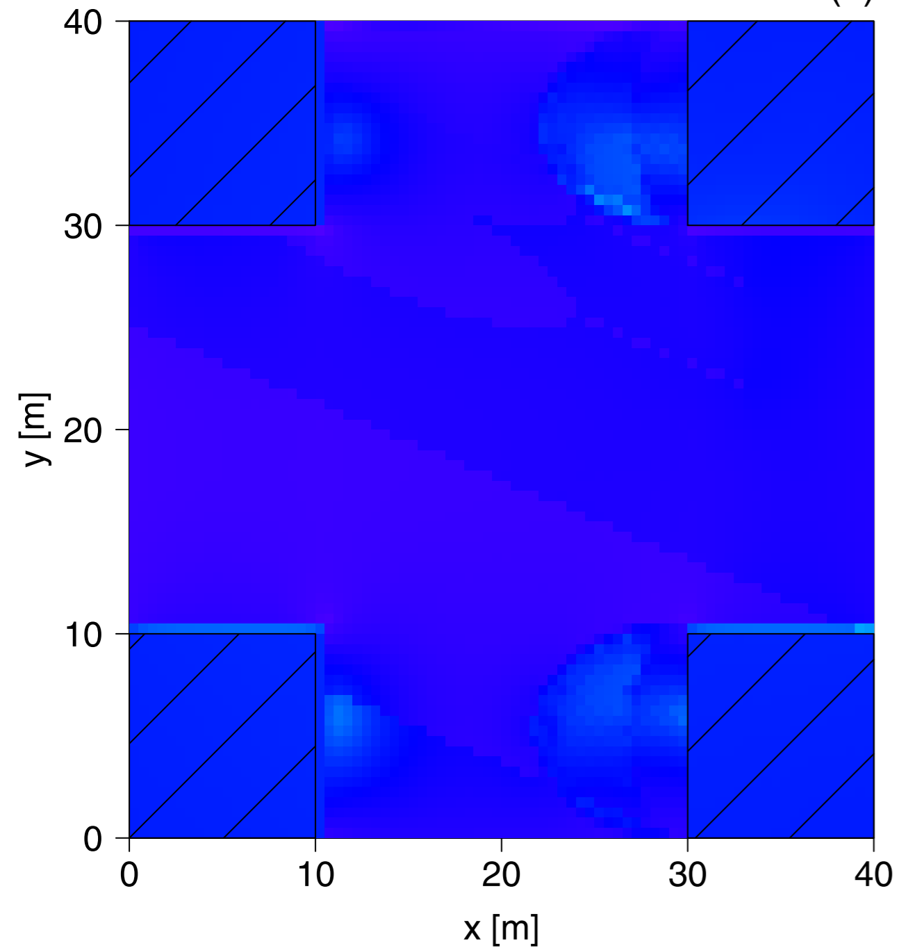
perct* [°C] as calculated by SkyHelios at 07:00 UTC
