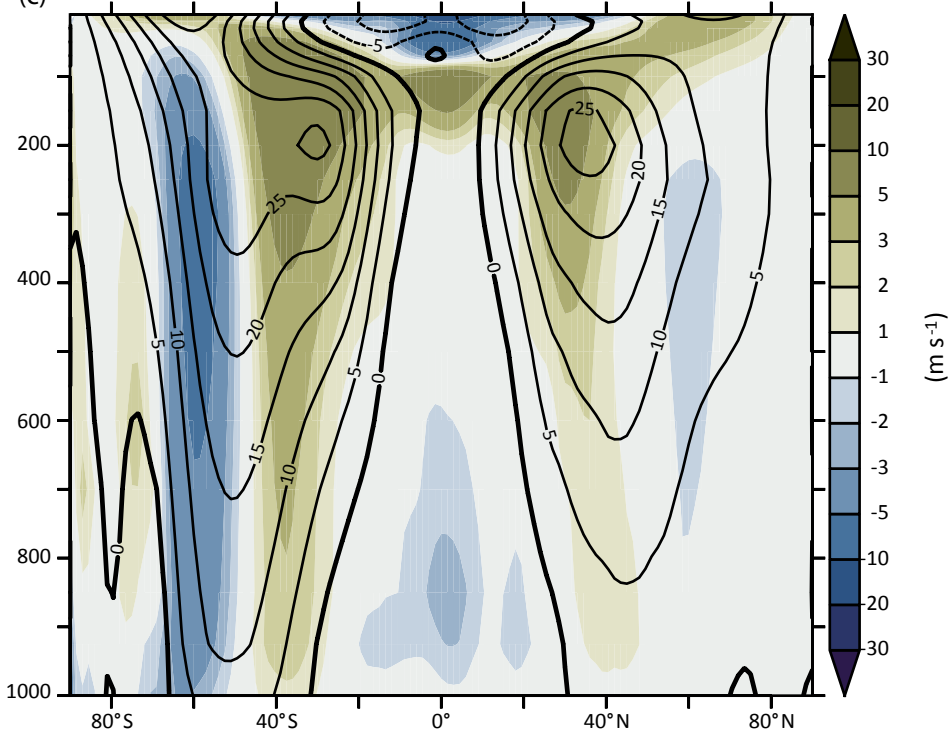
(c) Zonal wind : IPSL-CM5A2 - ERA-Interim
