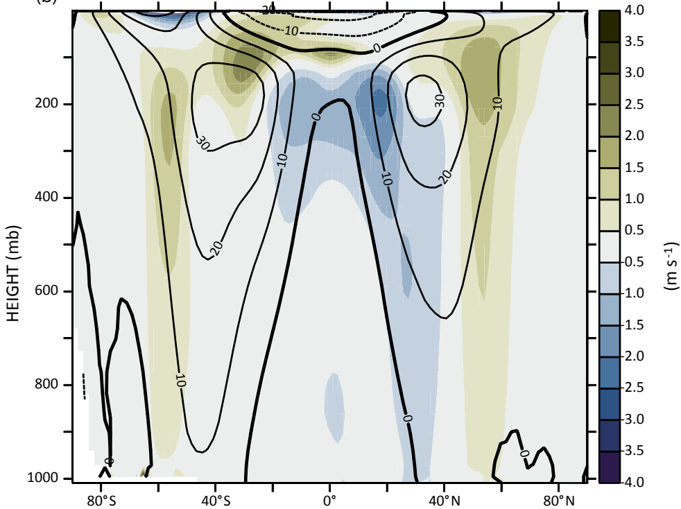
(c) Zonal wind : IPSL-CM5A2 - ERA-Interim
