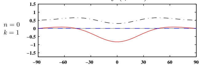
Rossby ( l_r = 1 )
