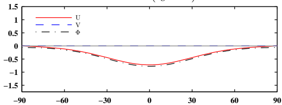
Kelvin ( l_e = 0 )
