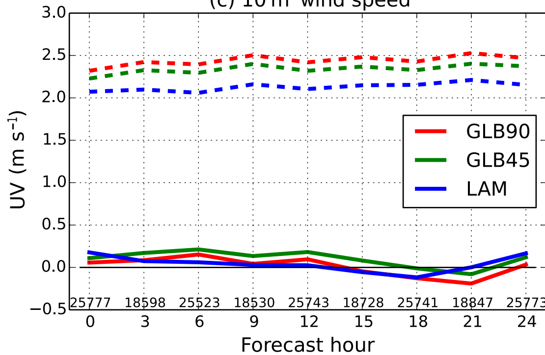
(c) 10 m wind speed
