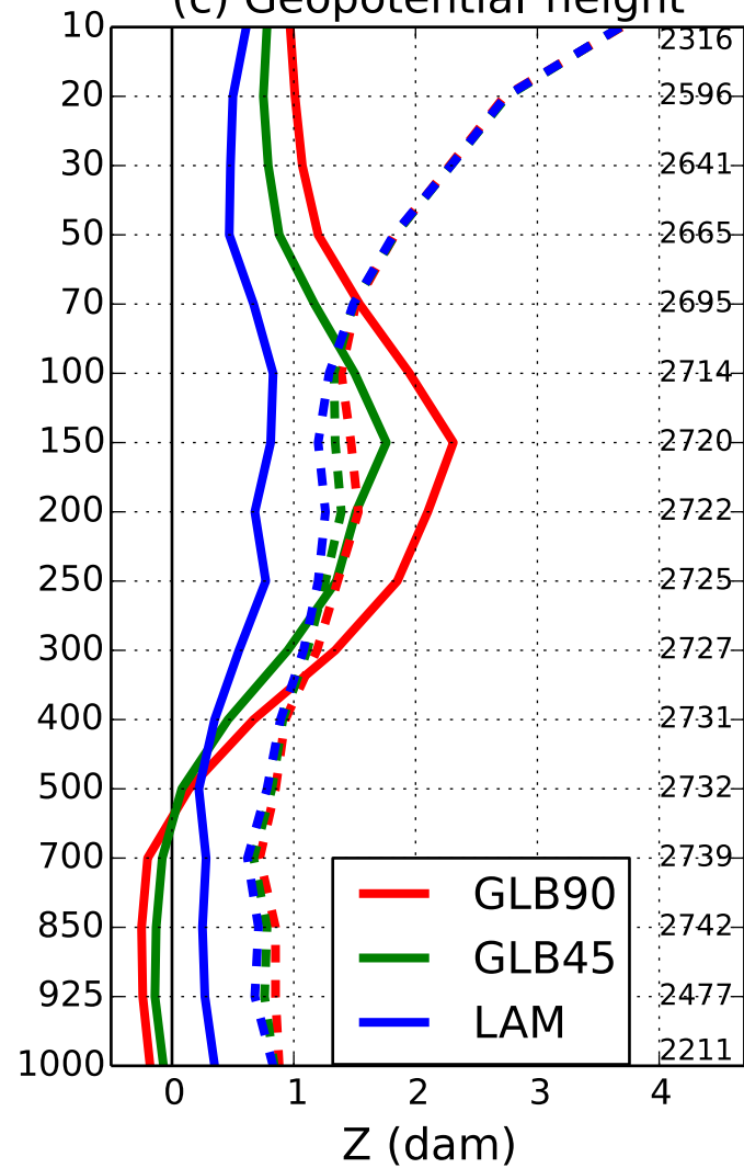
(c) Geopotential height
