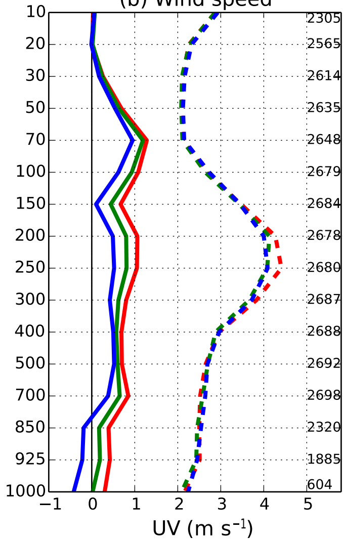
(b) Wind speed
