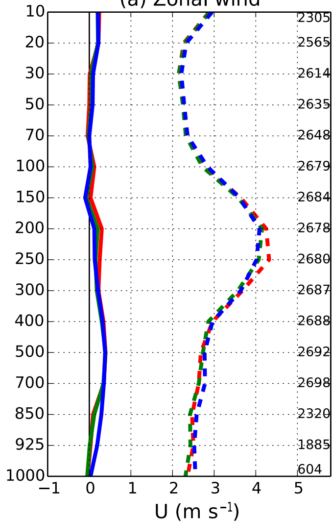
(a) Zonal wind
