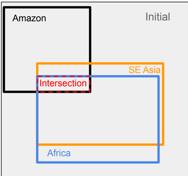
(a) Before bias correction
