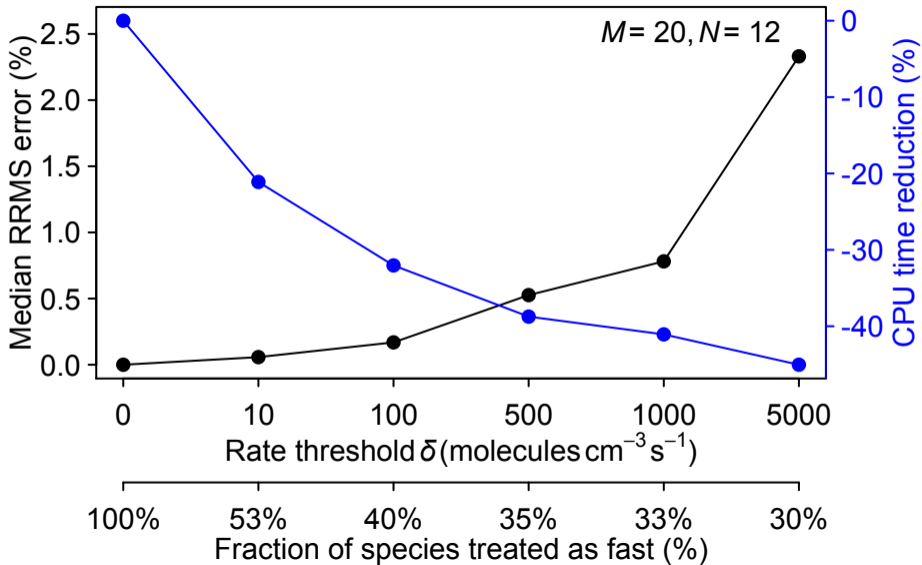
Performance and accuracy for different rate thresholds \delta
