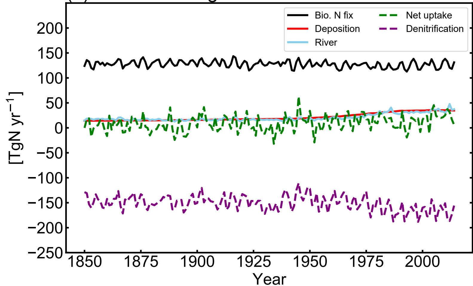
(b) Ocean N budget
