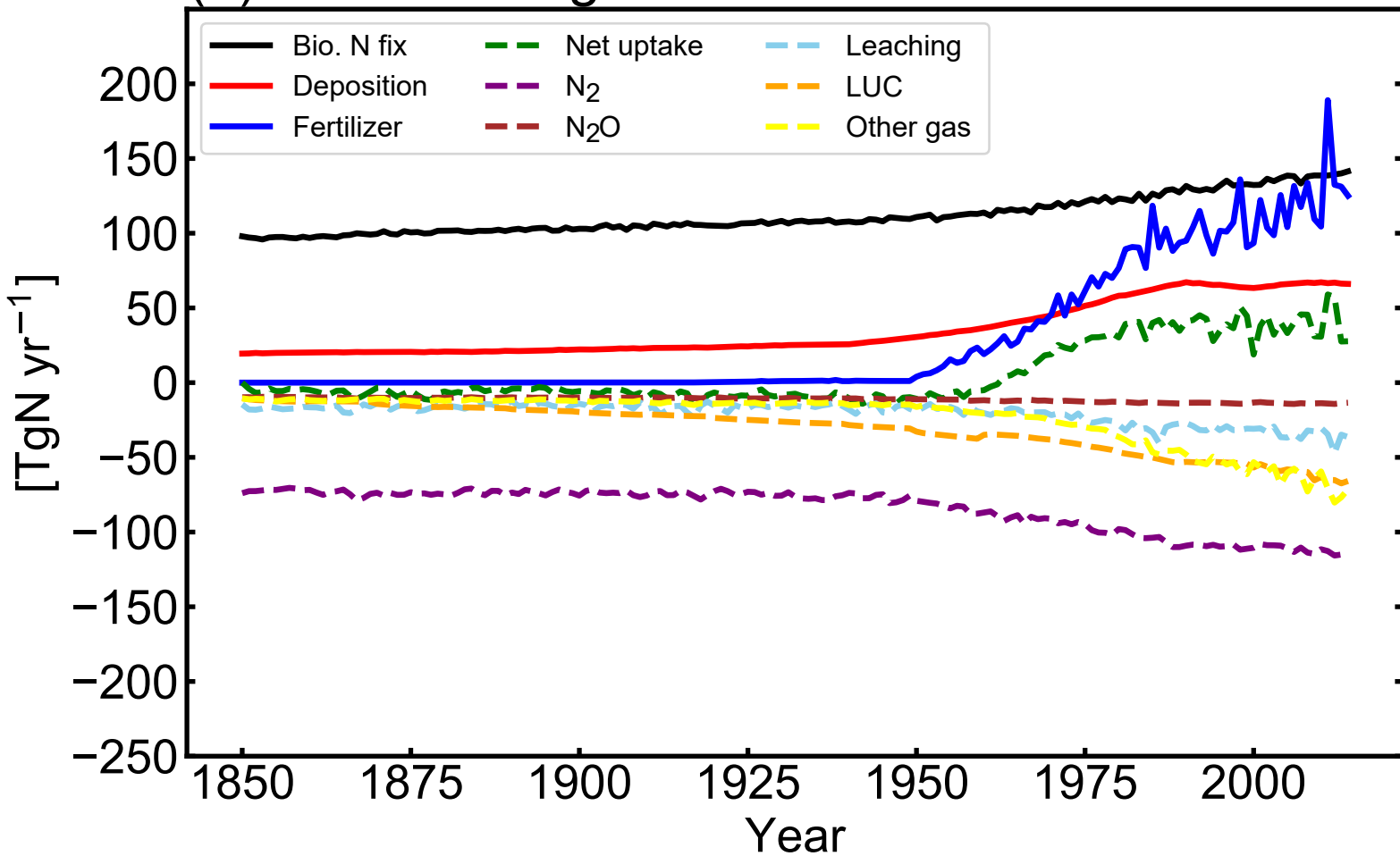
(a) Land N budget
