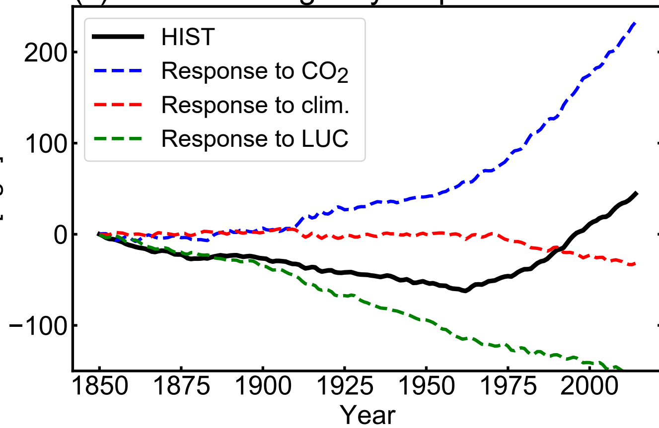
(c) Land C change: by responses
