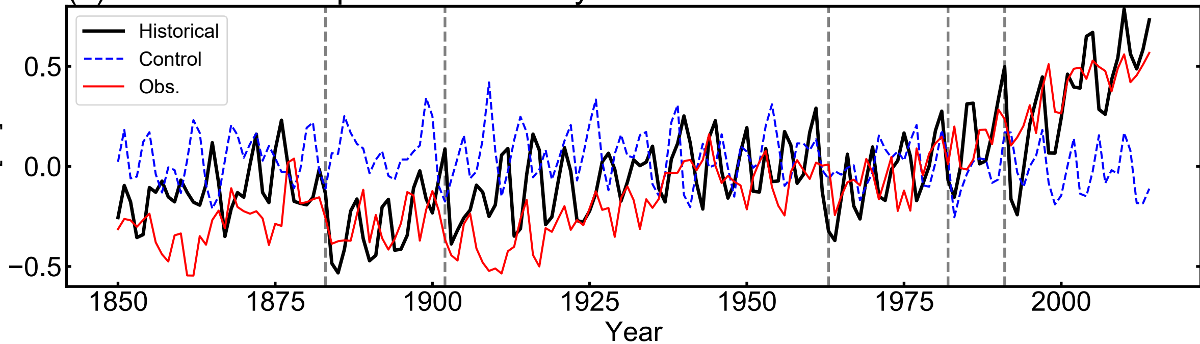
(c) Sea surface temperature anomaly
