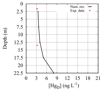
(c) Hg D concentration (station 12)
