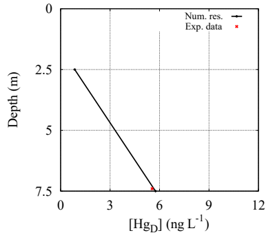
(f) Hg D concentration (station 26)
