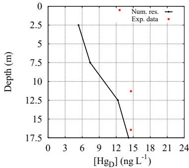
(e) Hg D concentration (station 20)
