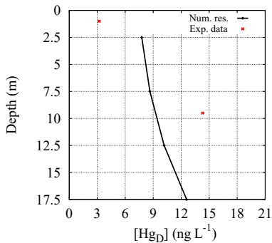
(b) Hg D concentration (station 10)
