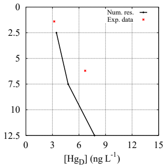
(a) Hg D concentration (station 1)
