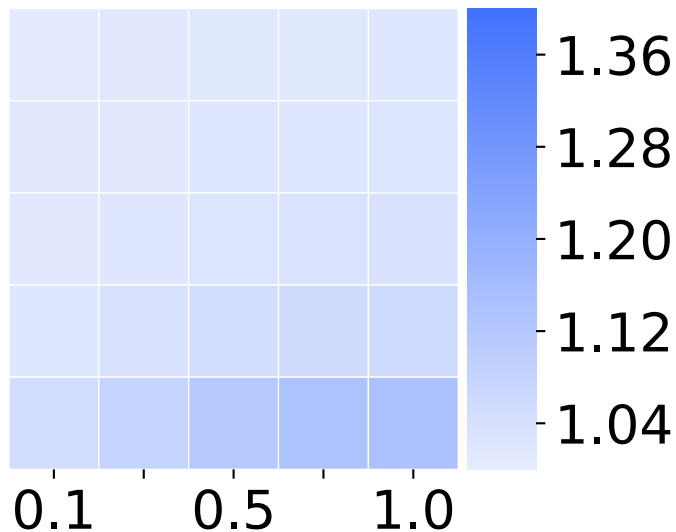
Spread ratio
