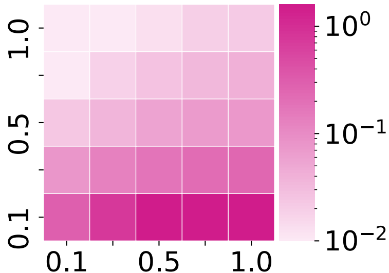
RMSE difference
