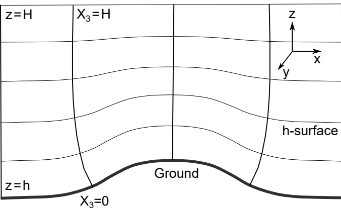
Vertical sigma coordinates (linear decay)
