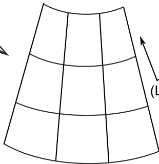
Vertical sigma coordinates (linear decay)
