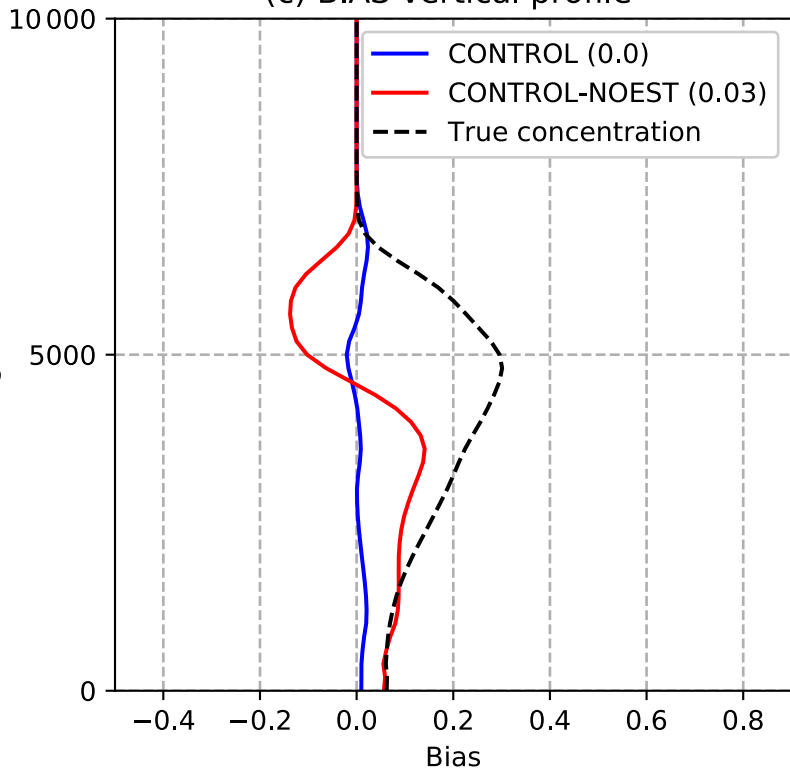
(c) BIAS vertical profile
