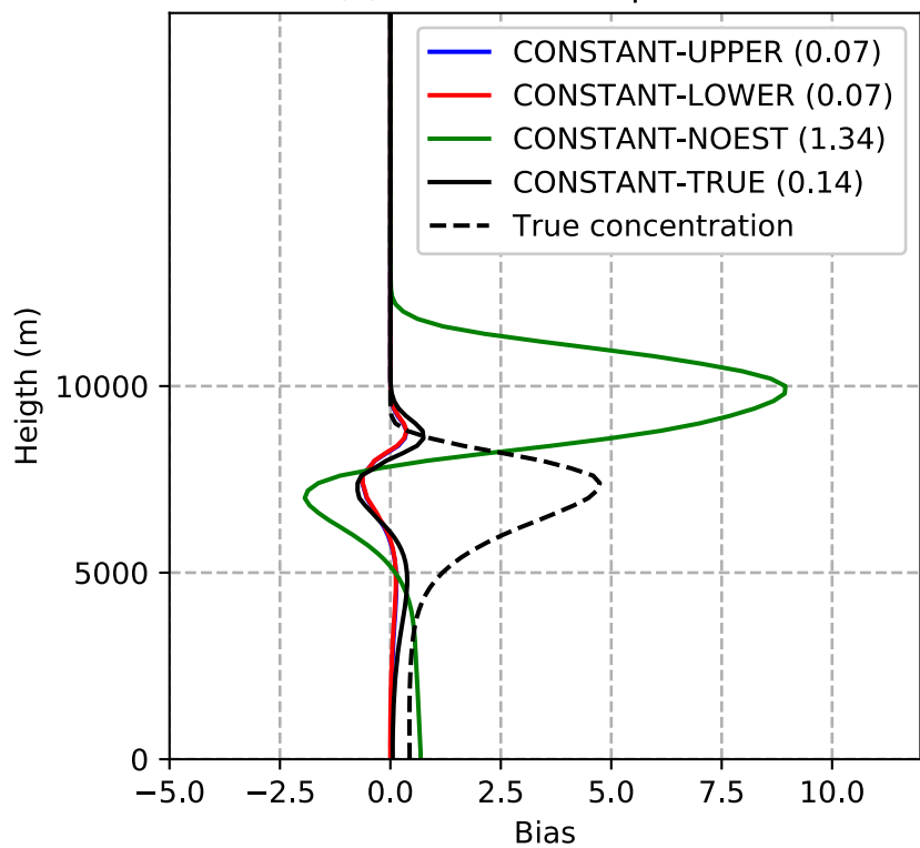
(c) BIAS vertical profile
