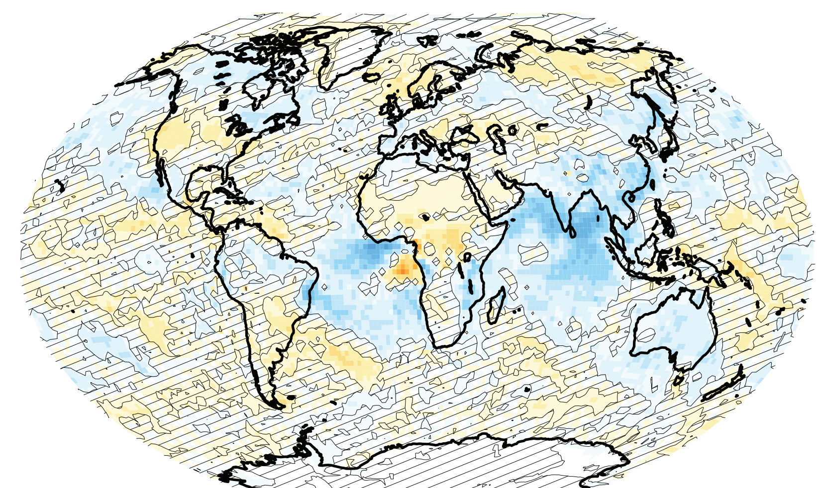
(c) Effective radiative forcing
