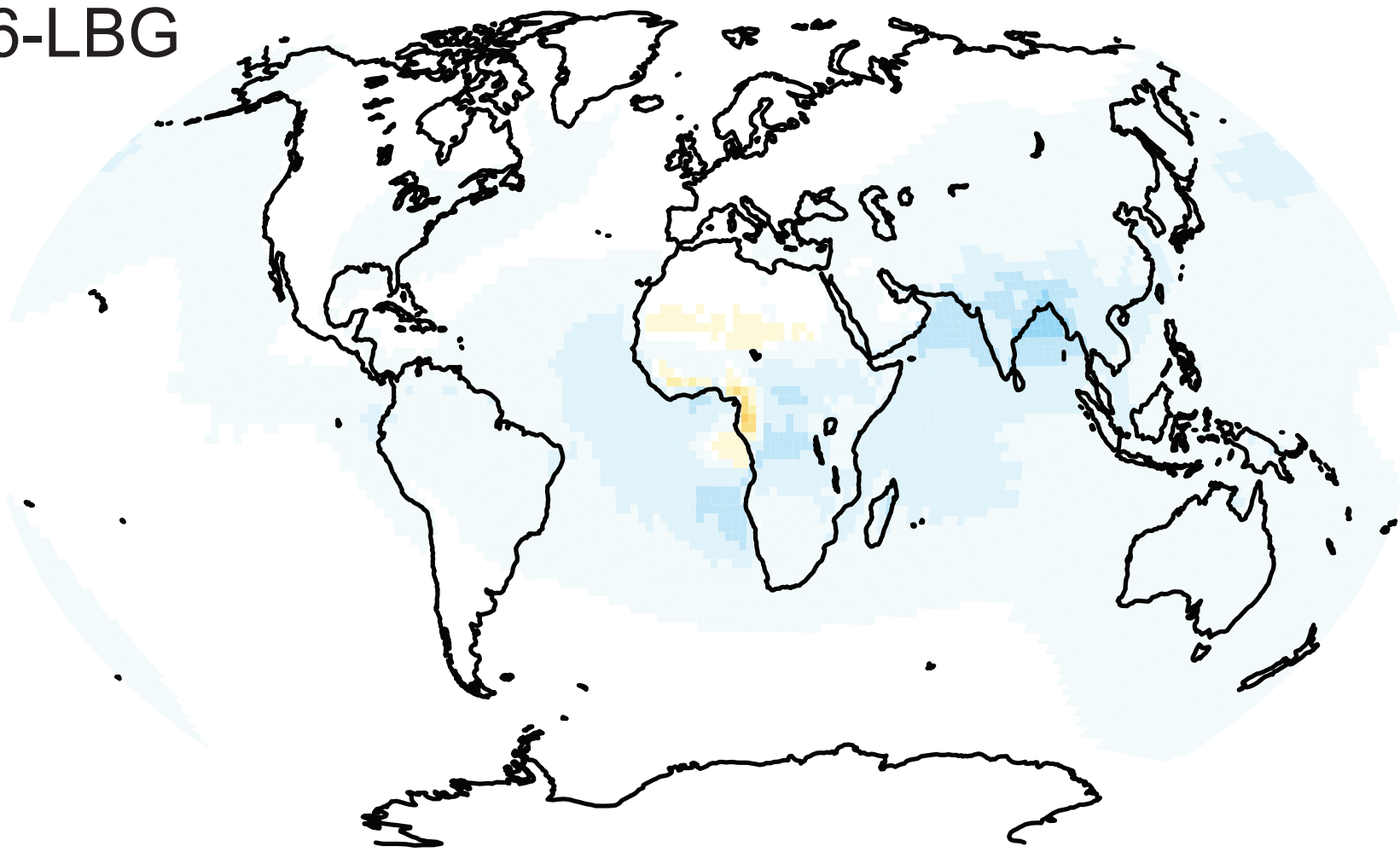
(a) Instantaneous radiative forcing
