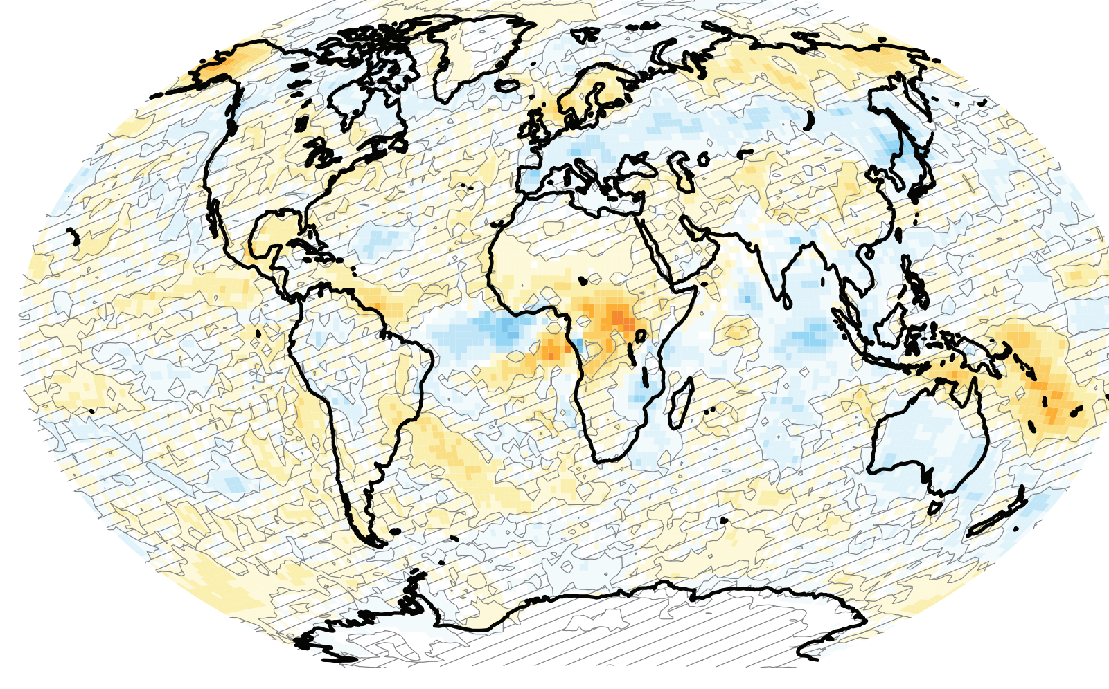
(b) Net rapid adjustments
