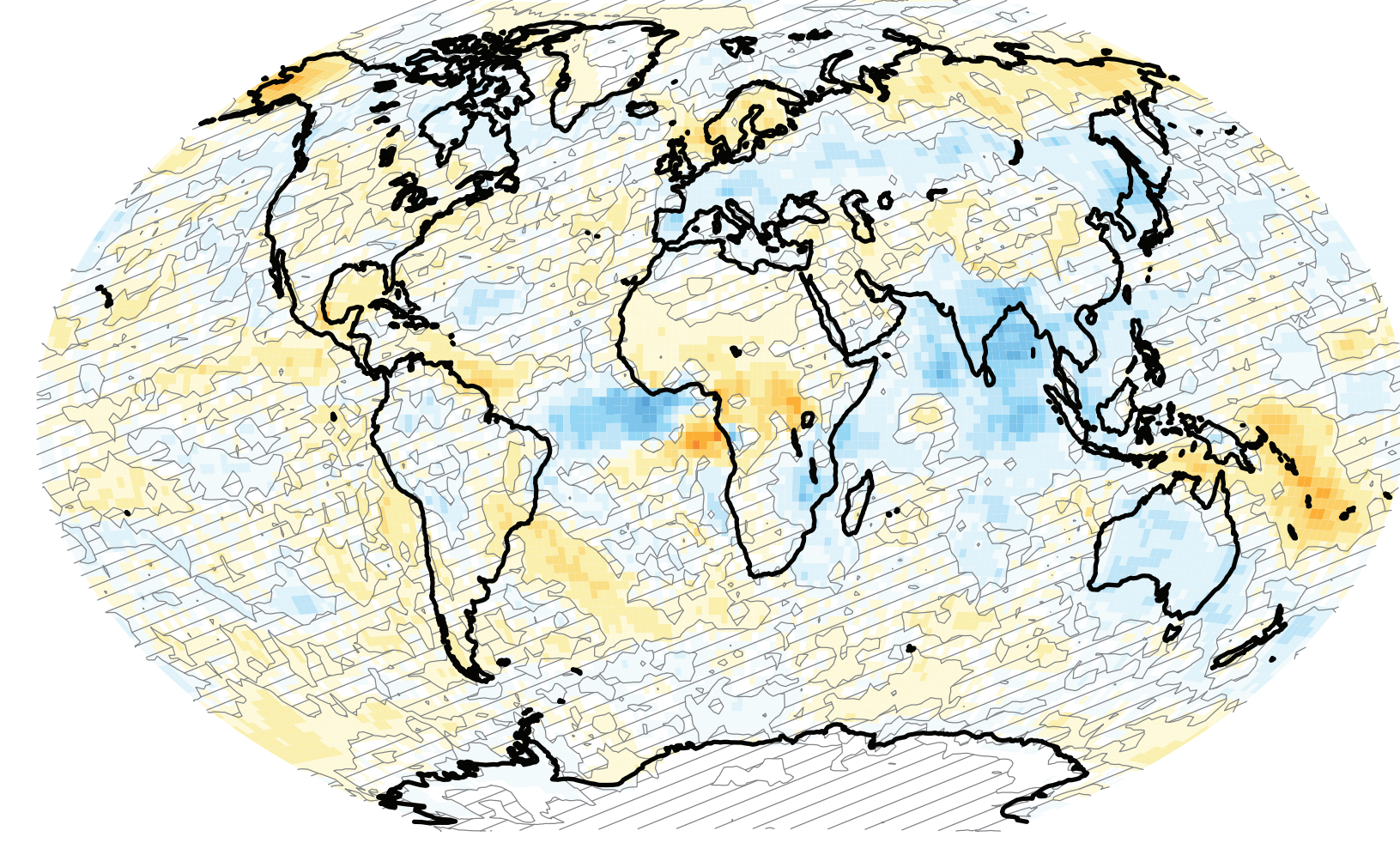
(c) Effective radiative forcing
