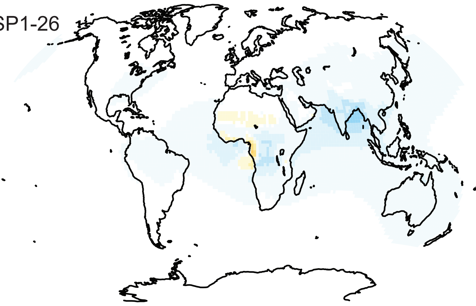
(a) Instantaneous radiative forcing
