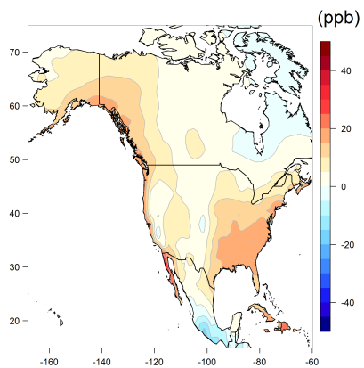
(f) MRIESM1r1
