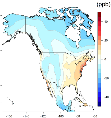
(a) CHASER
