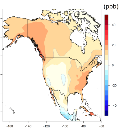
(c) GFDL-AM3
