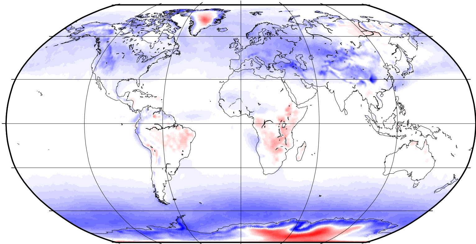
EC-Earth-Cloud_cci
