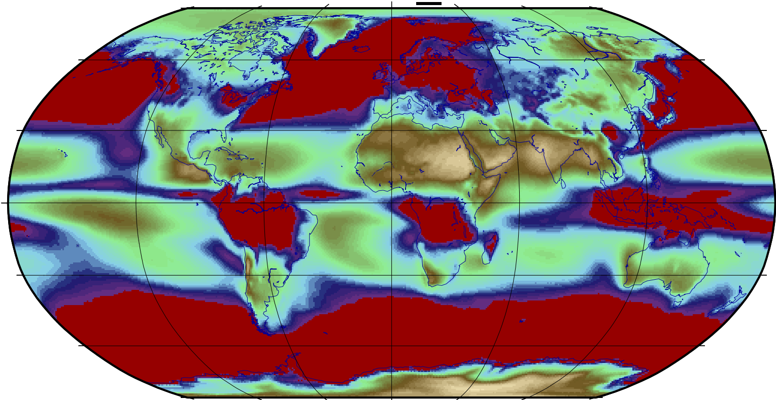
Cloud_cci
