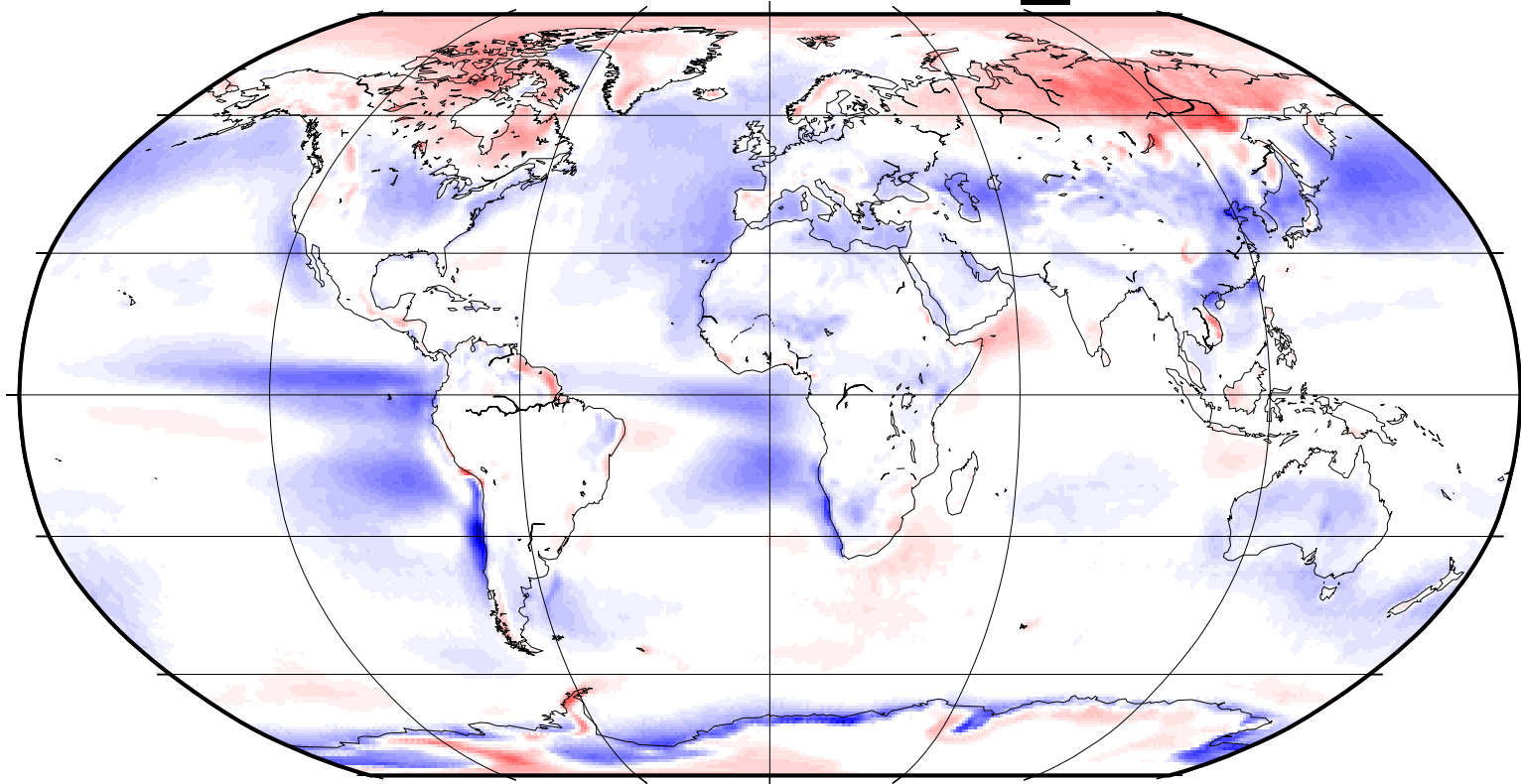
EC-Earth-Cloud_cci
