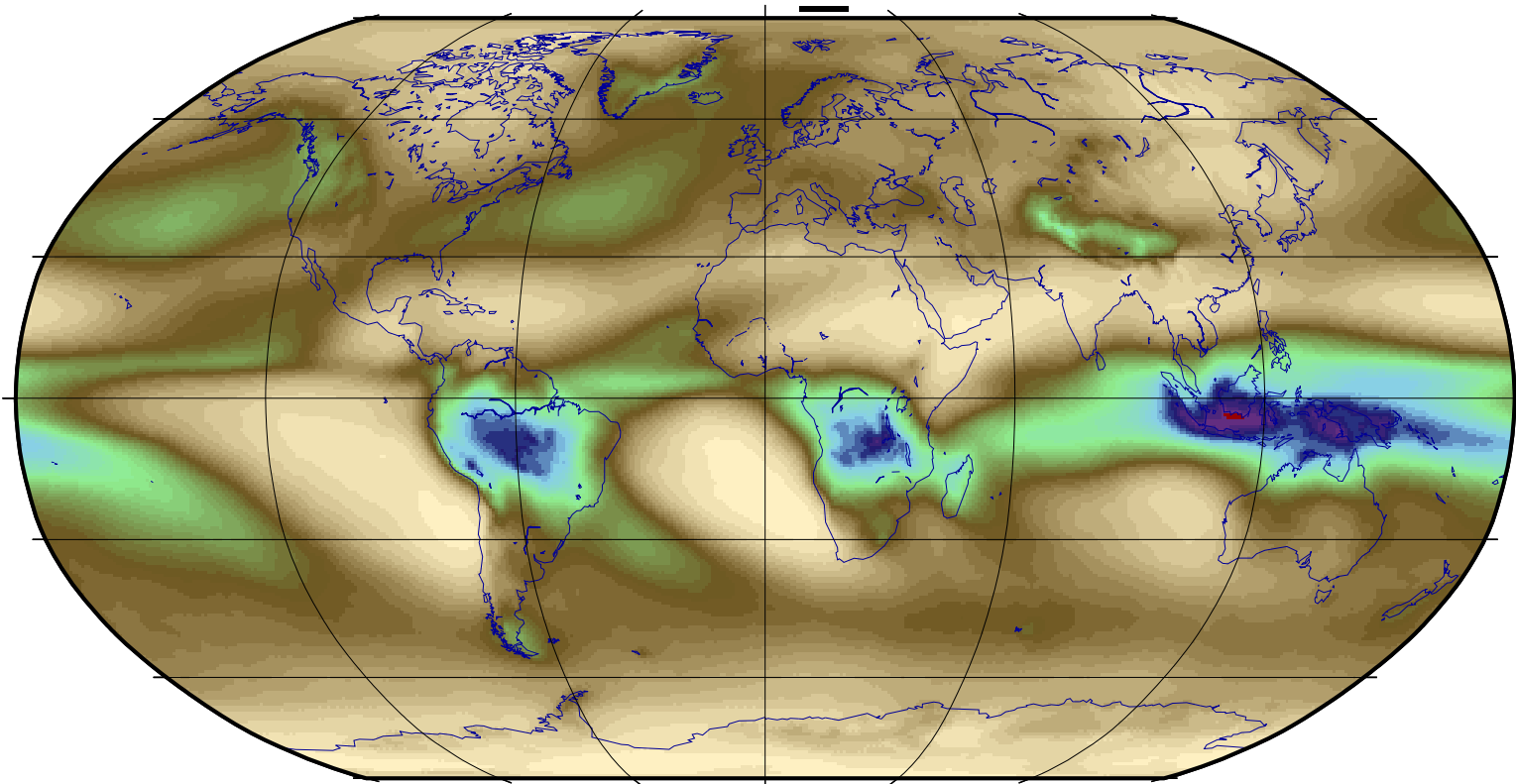
Cloud_cci
