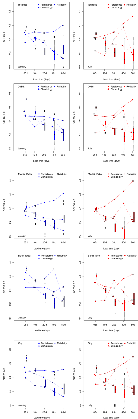
Figure 7. Skill scores for mean daily temperature in Toulouse and De Bilt, for lead times T of 5, 10, 20, 40, and 80 days. Squares indicate \text{CRPSS}_{\text{pers}} , triangles \text{CRPSS}_{\text{clim}} , and circles correlation. The diamonds indicate the reliability of CRPS (on the same scale as CRPSS). Blue symbols (left) are for January and red symbols (right) are for July. Triangles are identical for January and July. The boxplots for the correlation indicate the spread across the 100-member ensemble forecasts. Skill scores for temperature in Madrid and Berlin (continued). Skill scores for temperature in Orly (continued).
