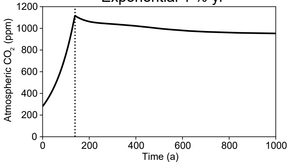
Exponential 1 % yr -1
