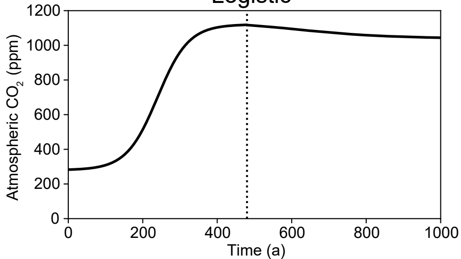
Logistic
