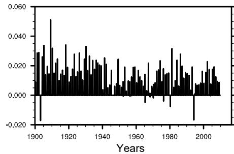
FH2OSFC (exice-cnt) [-]
