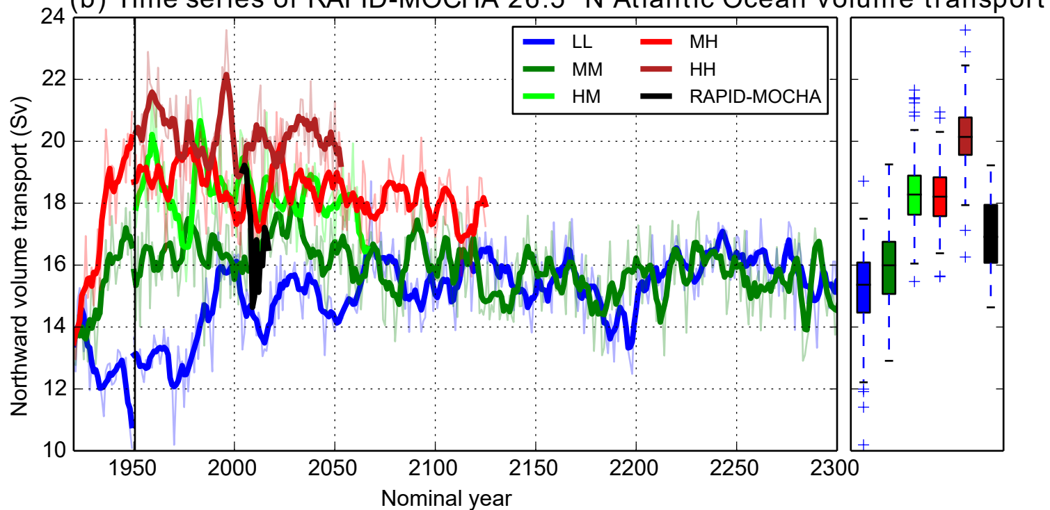
(b) Time series of RAPID-MOCHA 26.5° N Atlantic Ocean volume transport
