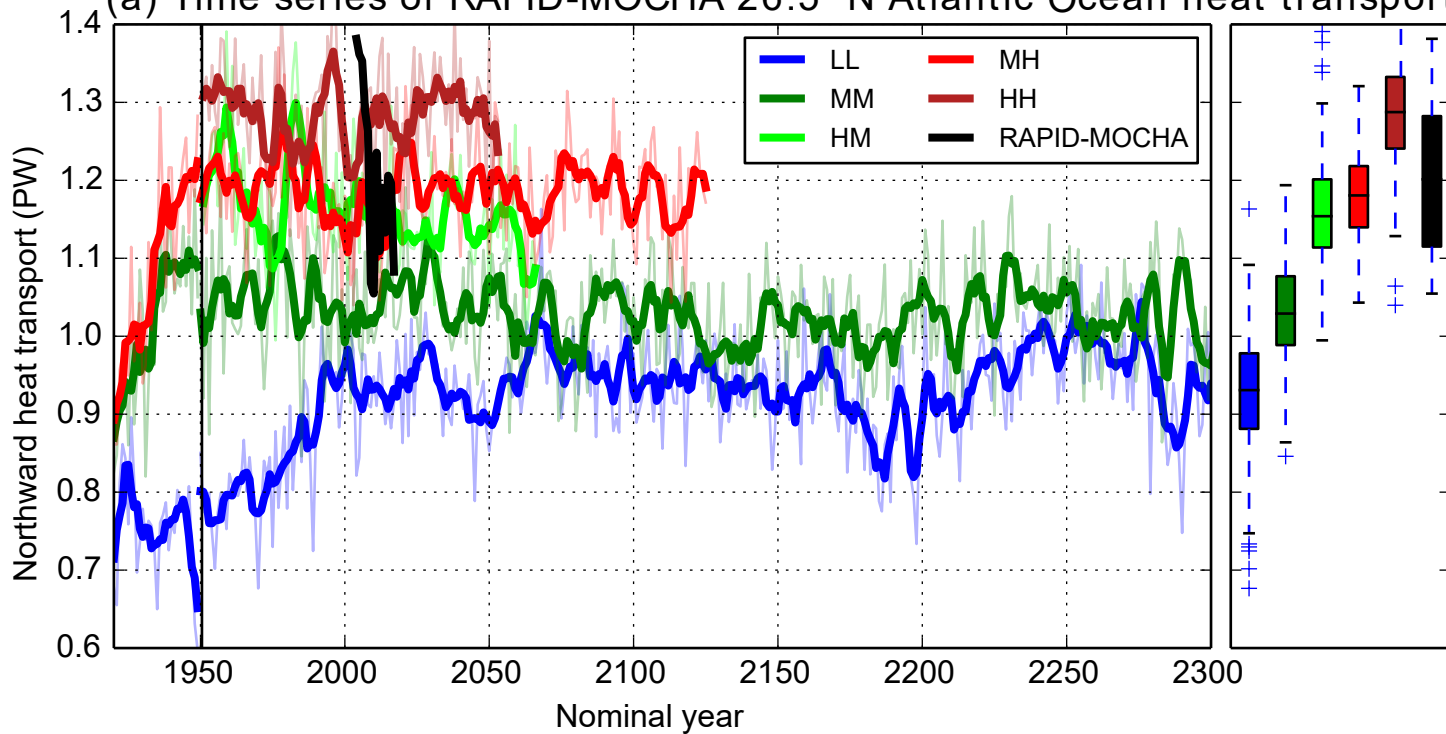
(a) Time series of RAPID-MOCHA 26.5° N Atlantic Ocean heat transport
