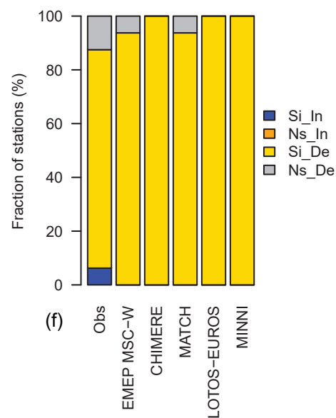
TNO 3 1990–2010 (PT)
