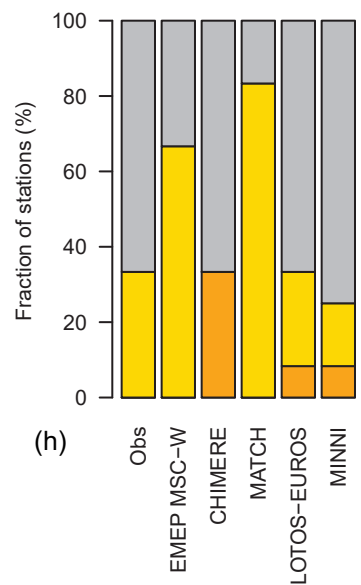
TNO 3 2000–2010 (P2)
