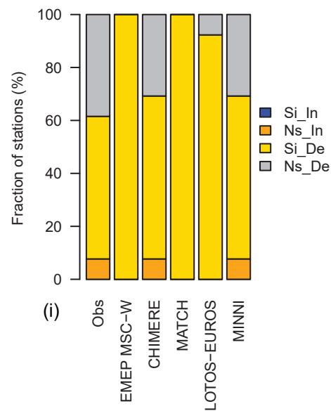
TNO 3 1990–2010 (PT)
