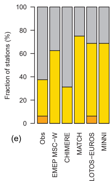
TNO 3 2000–2010 (P2)
