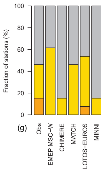
TNO 3 1990–2000 (P1)
