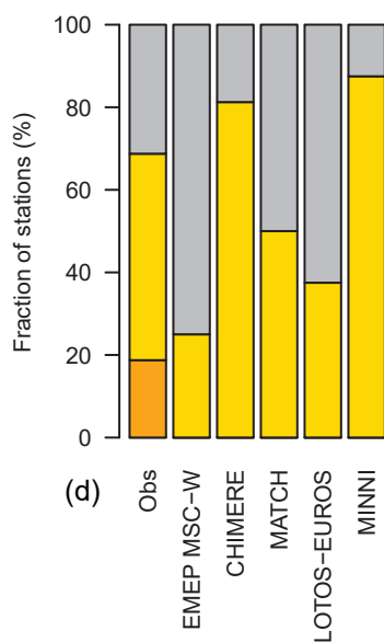
TNO 3 1990–2000 (P1)
