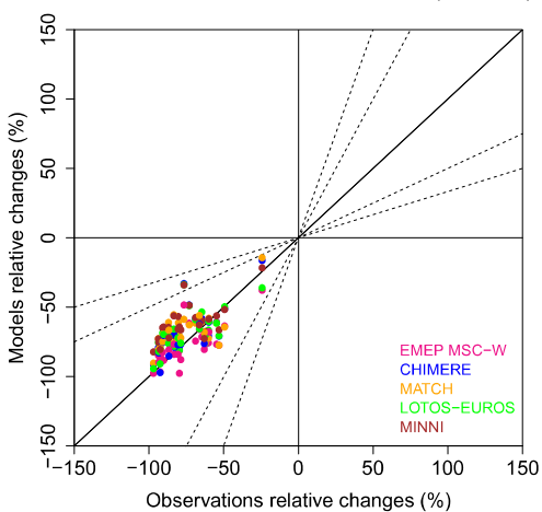
SO 2 relative trend at available EMEP sites (1990–2000)
