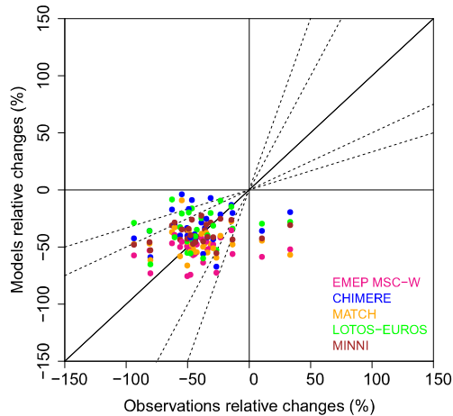
SO 2 relative trend at available EMEP sites (2000–2010)
