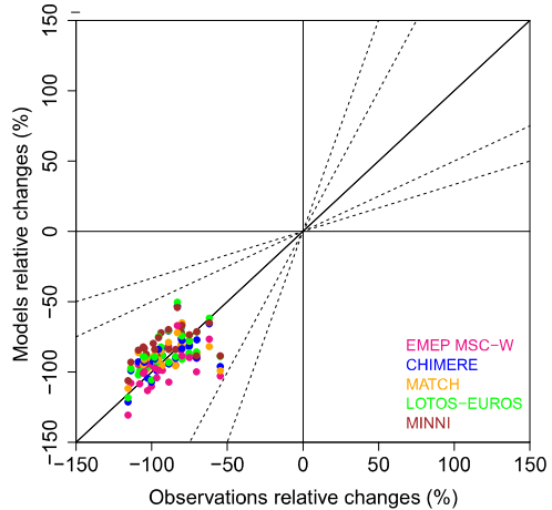
SO 2 relative trend at available EMEP sites (1990–2010)
