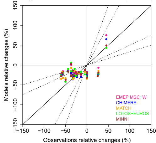
NO 2 relative trend at available EMEP sites (1990–2000)
