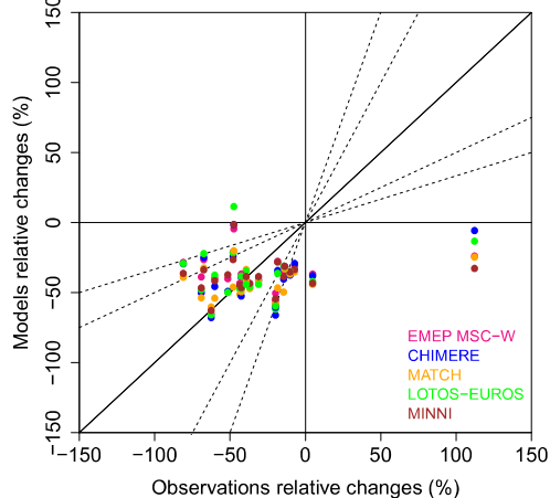
NO 2 relative trend at available EMEP sites (1990–2010)
