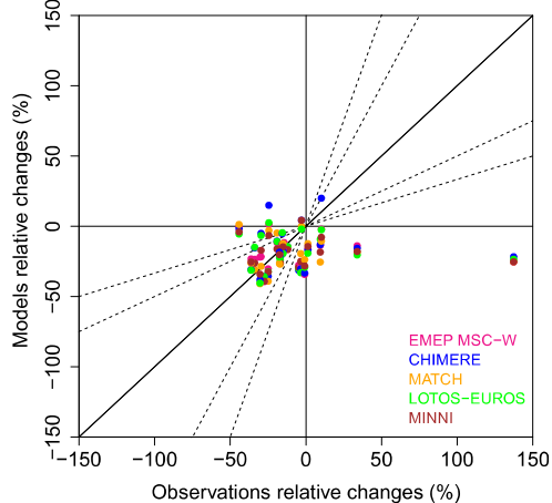
NO 2 relative trend at available EMEP sites (2000–2010)
