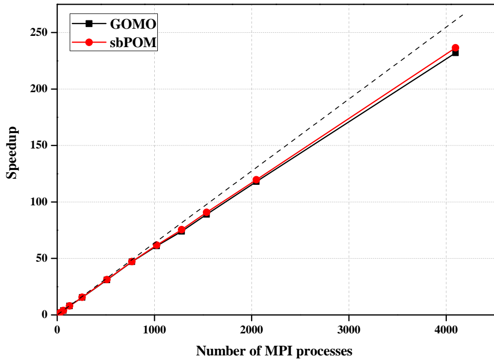
(a) Strong scaling
