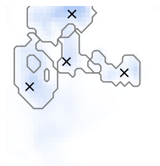
(e) Cloud volumes
