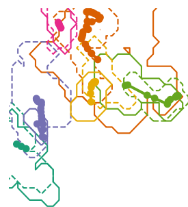
(f) Tracked cells
