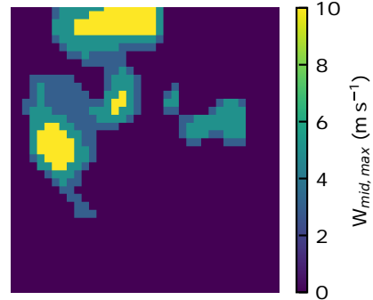
(f) Tracked cells
