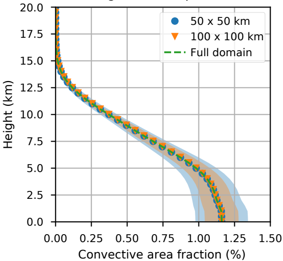
Avg \pm SD CAF profiles
