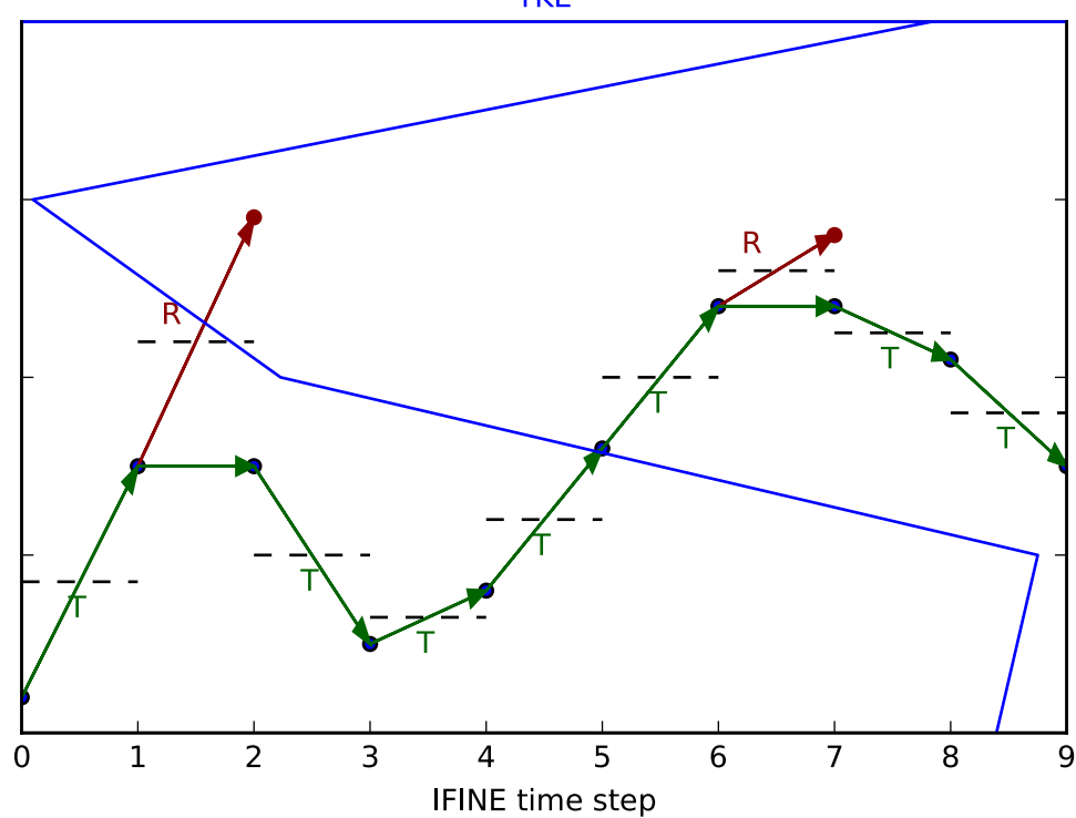
Small-discontinuity approximation
