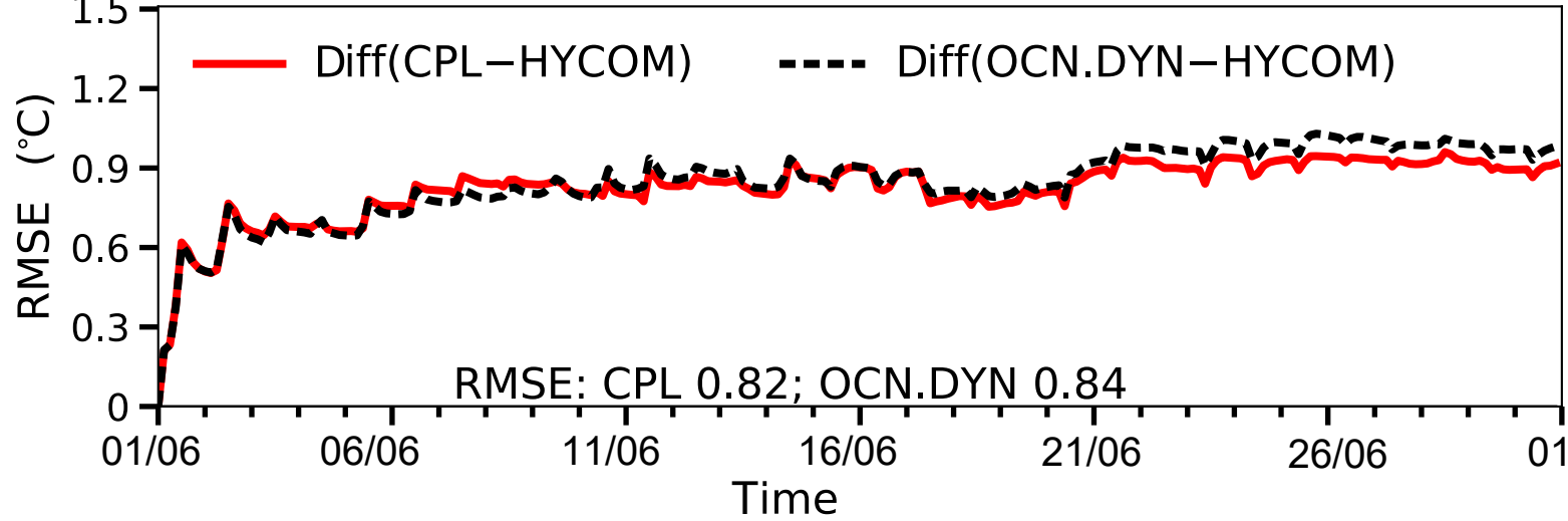
(a) Comparison with HYCOM
