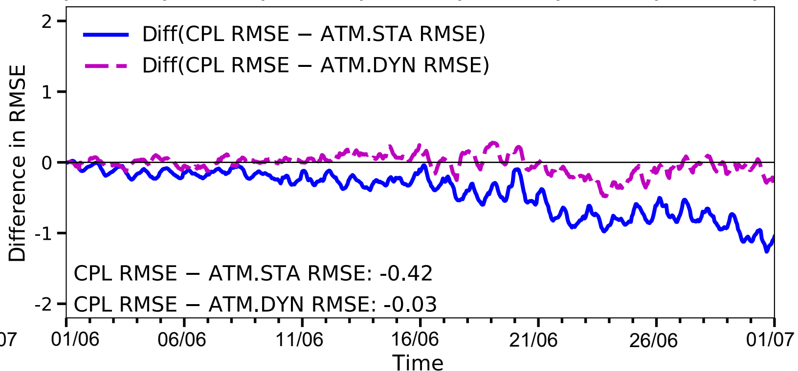
(b) RMSE between simulations and ERA5
