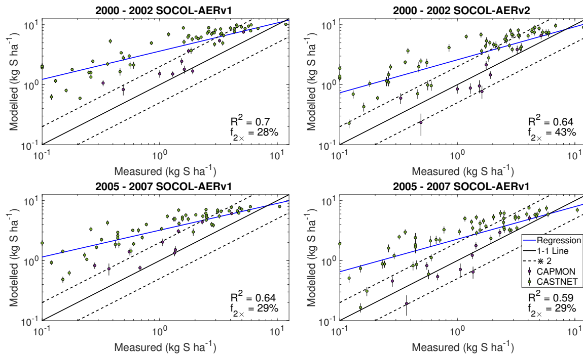
Figure S5: Evaluation of modelled SO 2 dry deposition against North American measurement sites from the WMO database (Vet et al., 2014). Socol-AERv1 and Socol-AERv2 are compared with measurements in two different time periods, 2000–2002 and 2005–2007. The ensemble standard deviation for the model results is shown as vertical bars. A power regression between the simulation results and measurements is shown in blue, and can be compared to the one-to-one line shown in black. Two model evaluation metrics are listed on the plots: the goodness of fit of the power regression between model and measurements ( R^2 ) and the fraction of sites for which the model is within a factor of 2 of measurements ( f_{2\times} ). Points are colored according to the measurement network of the sites.
