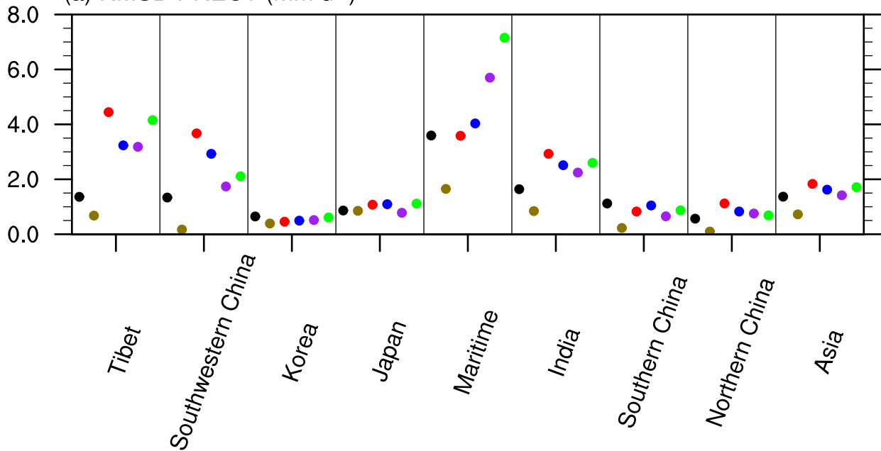
(a) RMSD PRECT (mm d -1 )
