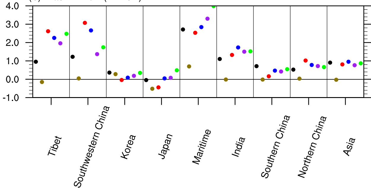
(b) Bias PRECT (mm d -1 )
