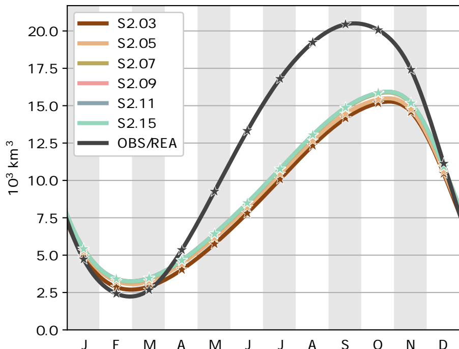
(b) Antarctic sea ice volume
