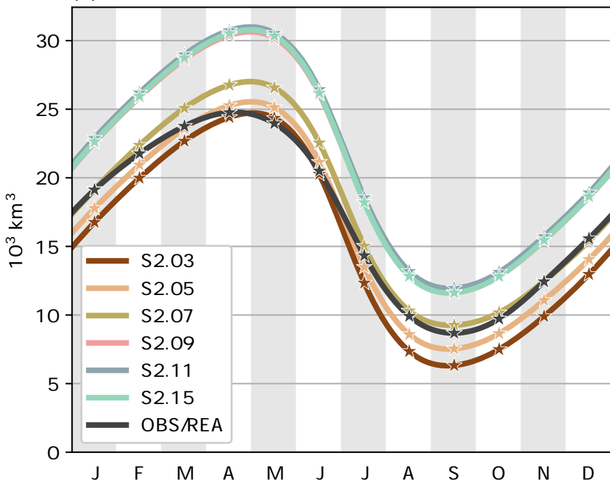
(a) Arctic sea ice volume
