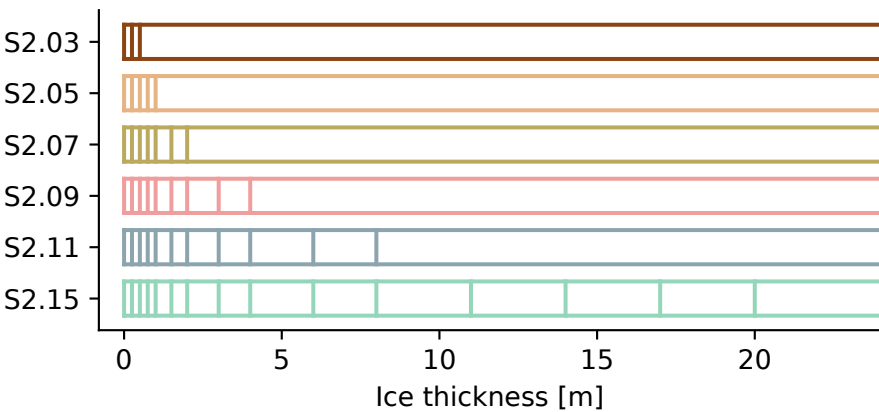
S2 - adding thick ice categories
