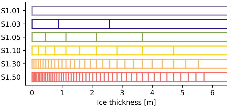
S1 - changing number and position of boundaries
