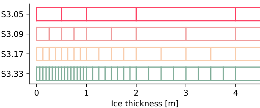
S3 - refining resolution within a fixed set of five categories
