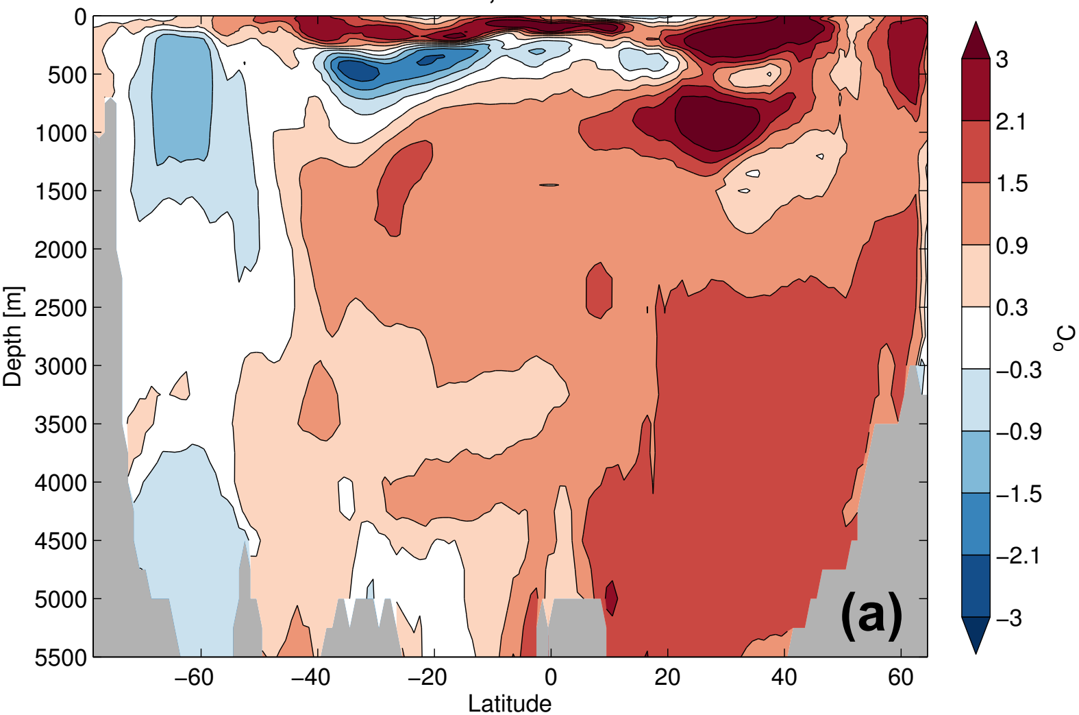
Atlantic zonal mean T, NorESM1-F minus WOA09
