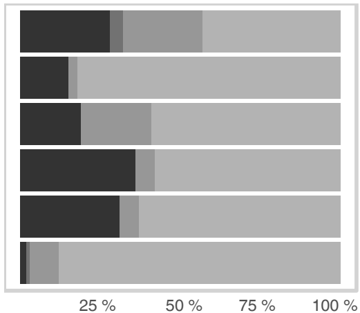
Observations : RL
