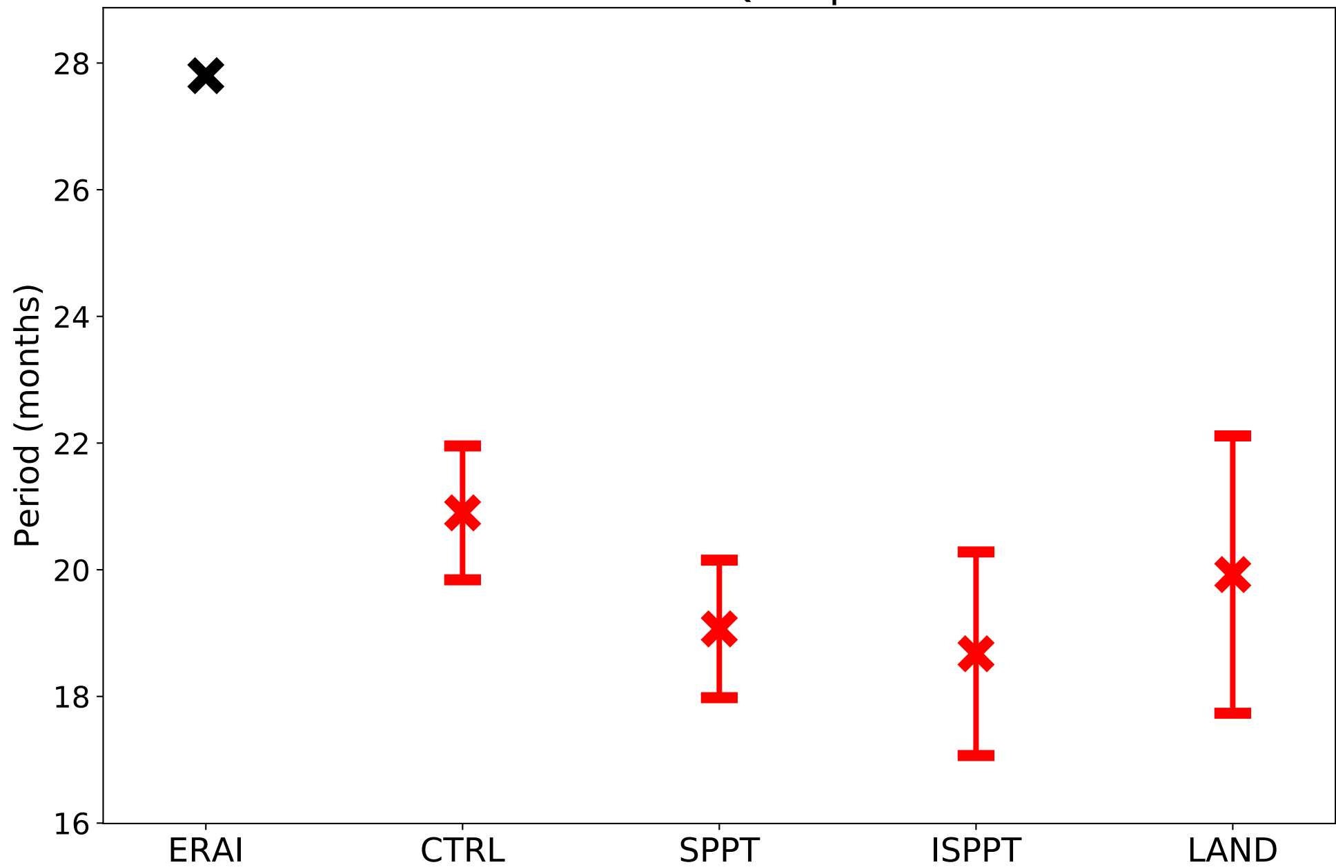
Estimate of QBO period
