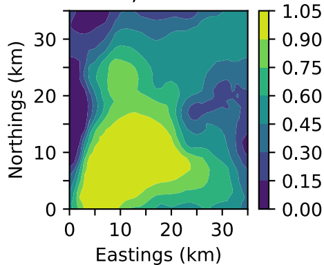
Run J, z = 3.5 km
