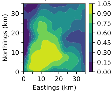
Run D, z = 3.5 km
