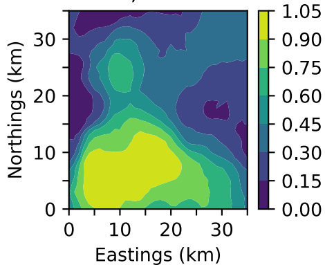
Run E, z = 3.5 km
