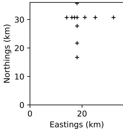
Magnetotelluric
