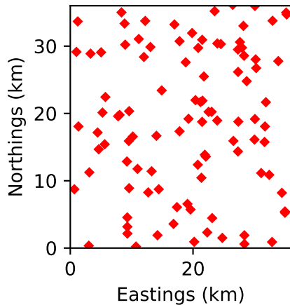
Magnetic anomaly
