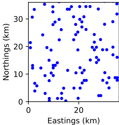
Gravity anomaly
