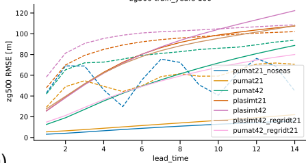
zg500 train_years 100
