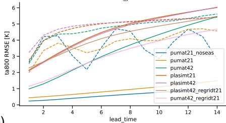
ta800 train_years 100
