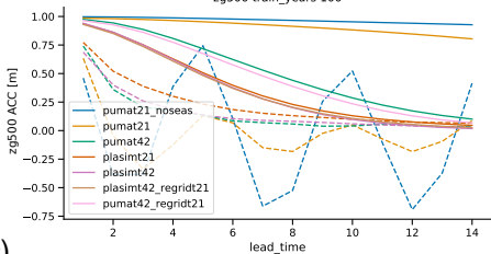
zg500 train_years 100
