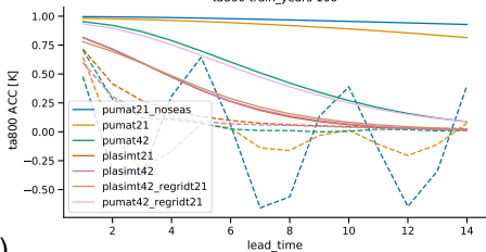
ta800 train_years 100
