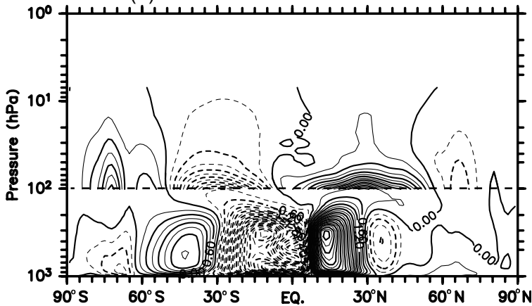
(b) Mass streamfunction in MIROC5
