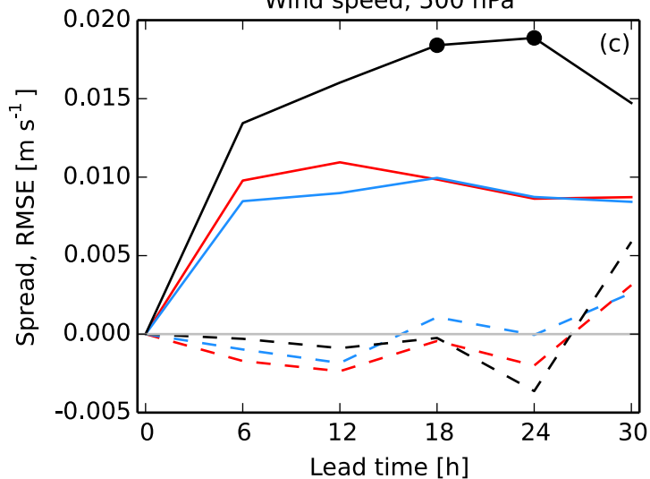
Wind speed, 500 hPa
