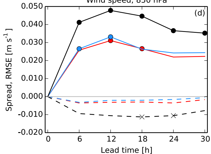
Wind speed, 850 hPa
