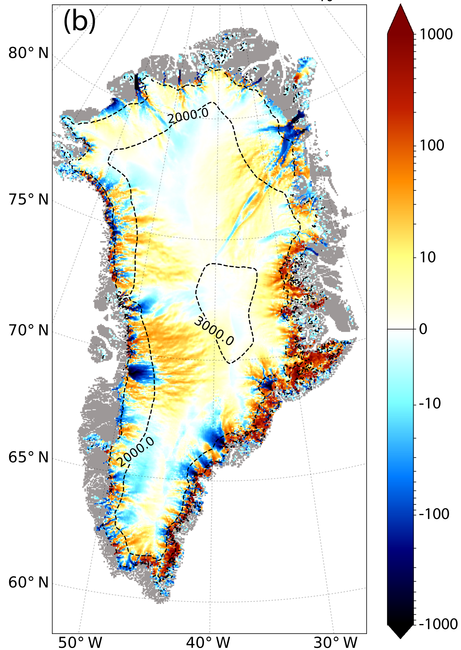
Ice velocity difference ( \text{Log}_{10} \text{ m yr}^{-1} )
