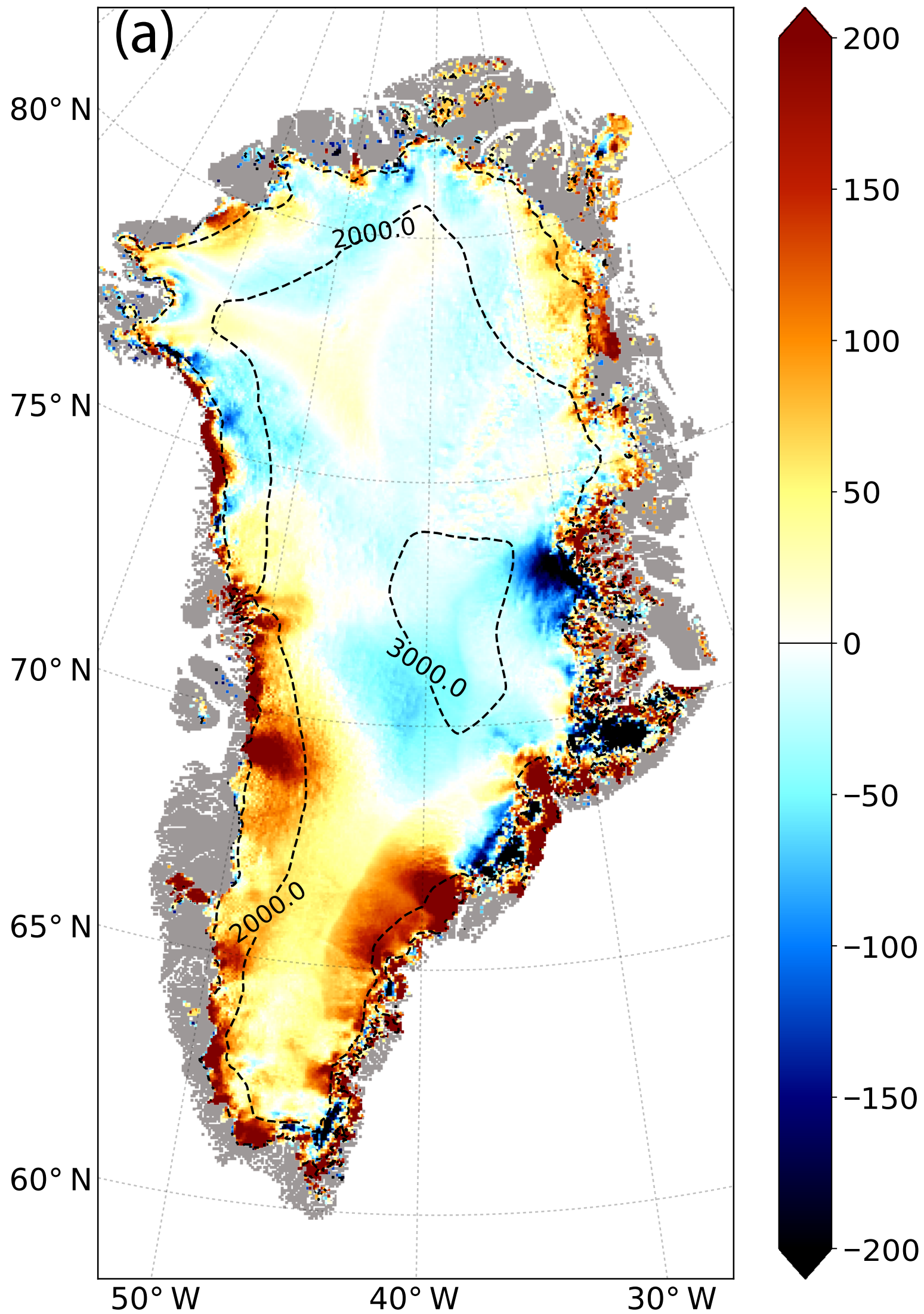
Ice thickness difference (m)
