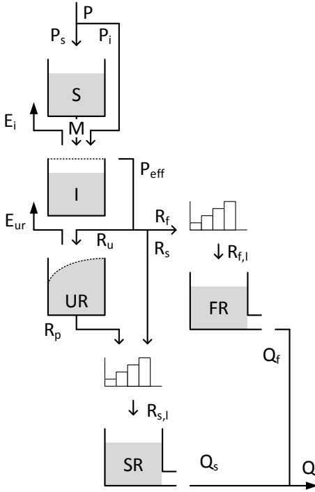
Figure S35: Structure of the FLEX-IS model
