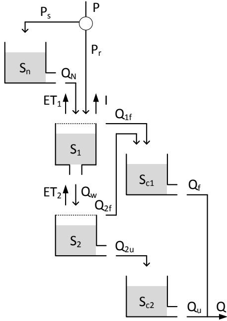
Figure S33: Structure of the MOPEX-4 model
