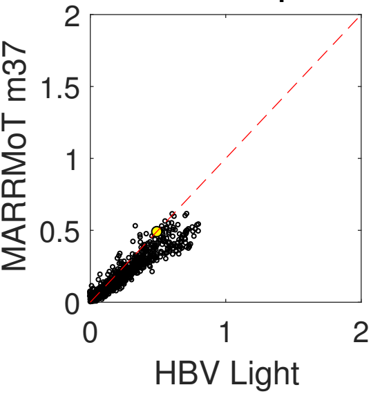
(c) KGE_r
