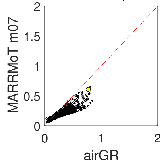
(f) KGE_r
