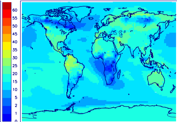
(b) Contribution to near-surface CH 3 COOH (%)
