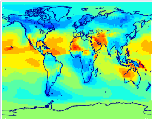
(a) Contribution to near-surface HCOOH (%)
