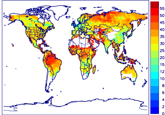
(b) 1,6 isom. fraction, C4-addition
