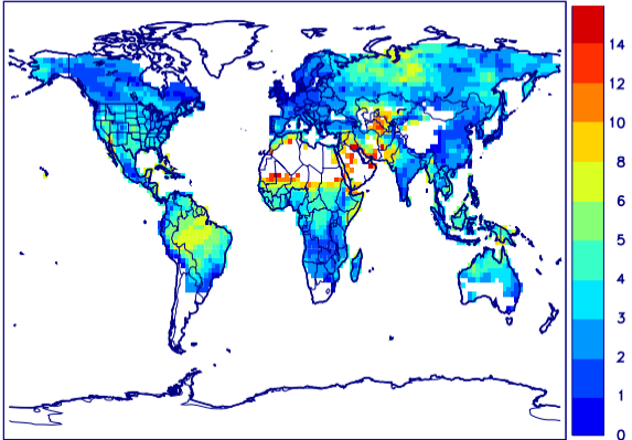
(a) 1,6 isom. fraction, C1-addition
