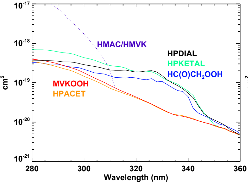
(a) Hydroperoxycarbonyls and keto-enols
