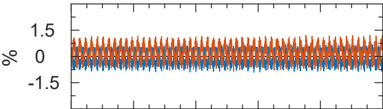
(a) Rossby
